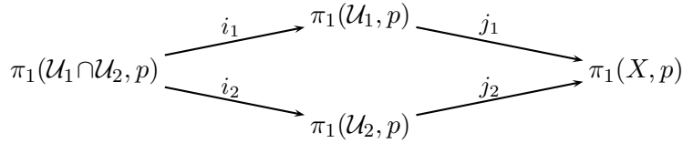
Figure 1: Van Kampen's Theorem Setting
