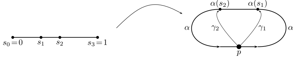
Figure 7: Splitting an Element of \mathcal{L}(X, p) into Elements of \mathcal{L}(\mathcal{U}_1, p) and \mathcal{L}(\mathcal{U}_2, p)
