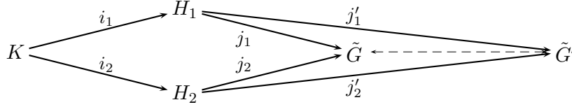
Figure 4: An Amalgated Product
